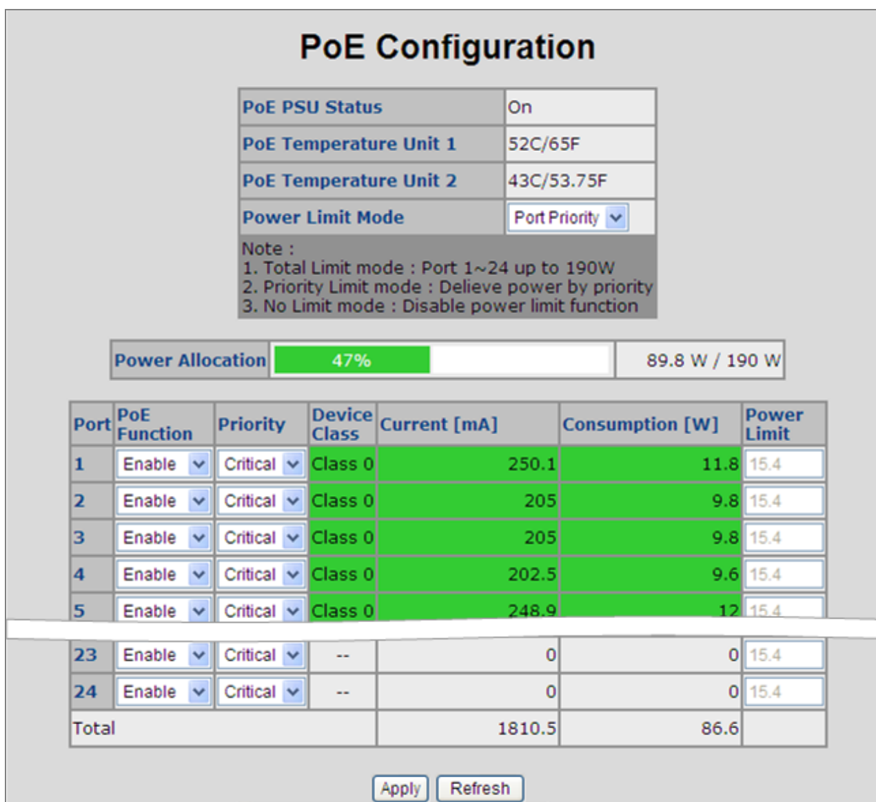
Figure 4-13-1: PoE Configuration
